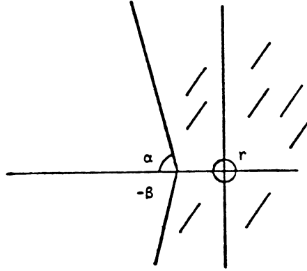
FIGURE 2. The set \mathcal{P}_\alpha
